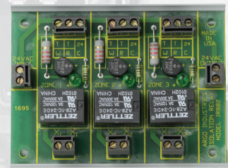
IR882 Isolation Relay
